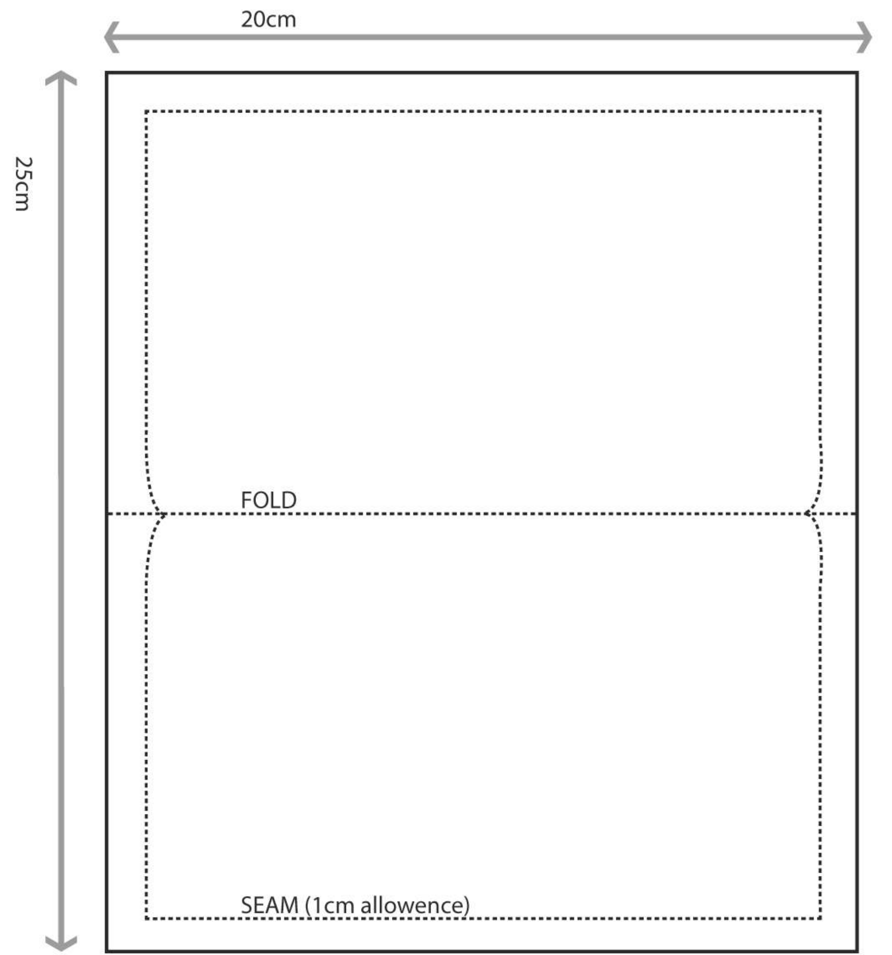
INTERNAL BAG SHELL X1
